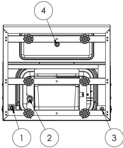
Bottom View
